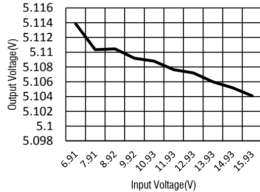
Line Regulation
