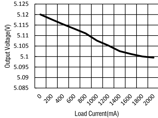
Load Regulation
